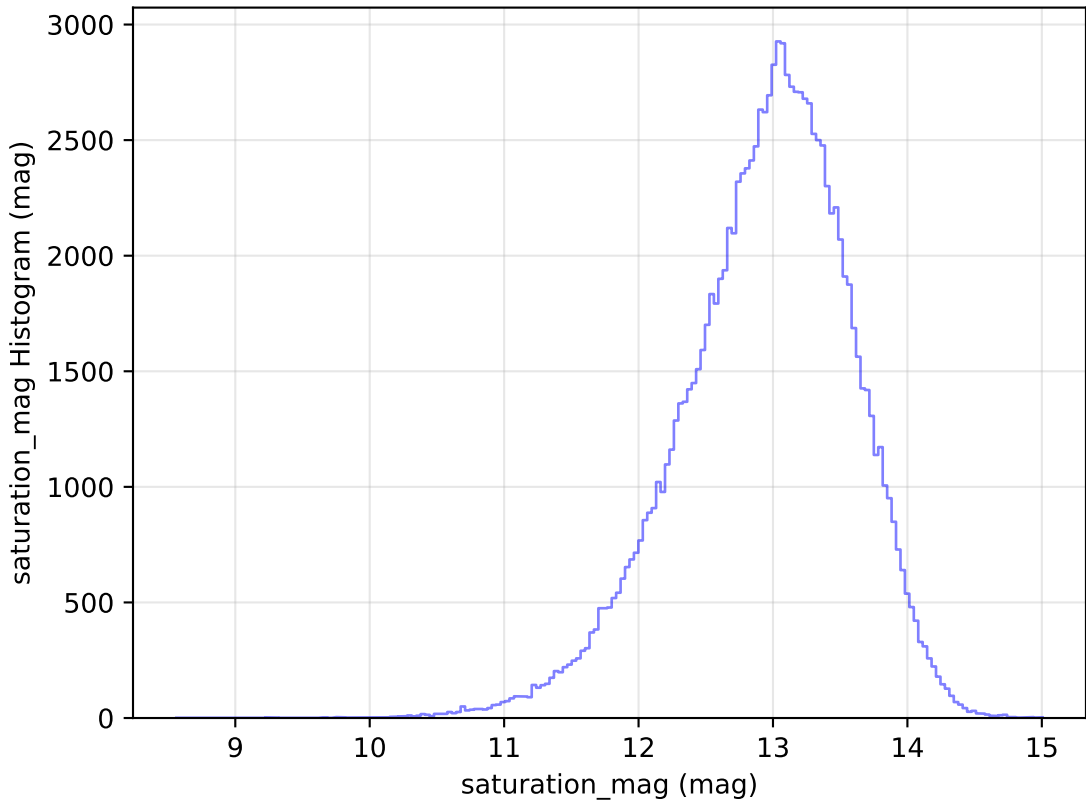
too_elab_r16_d2_giz_v3.4_10yrs WFD u band: saturation_mag Histogram
