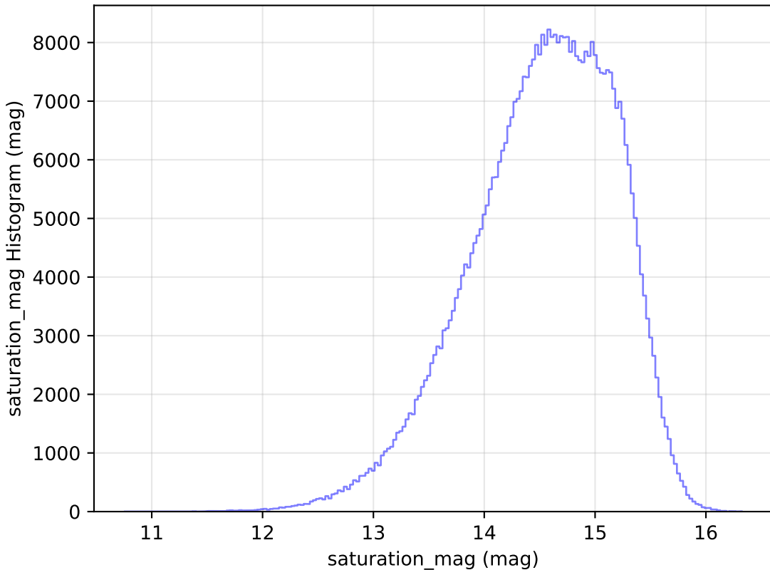
too_elab_r16_d2_giz_v3.4_10yrs WFD r band: saturation_mag Histogram
