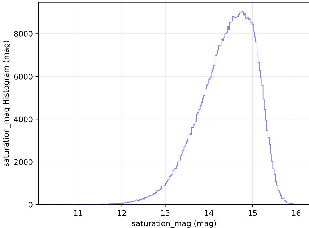
too_elab_r16_d2_giz_v3.4_10yrs WFD i band: saturation_mag Histogram
