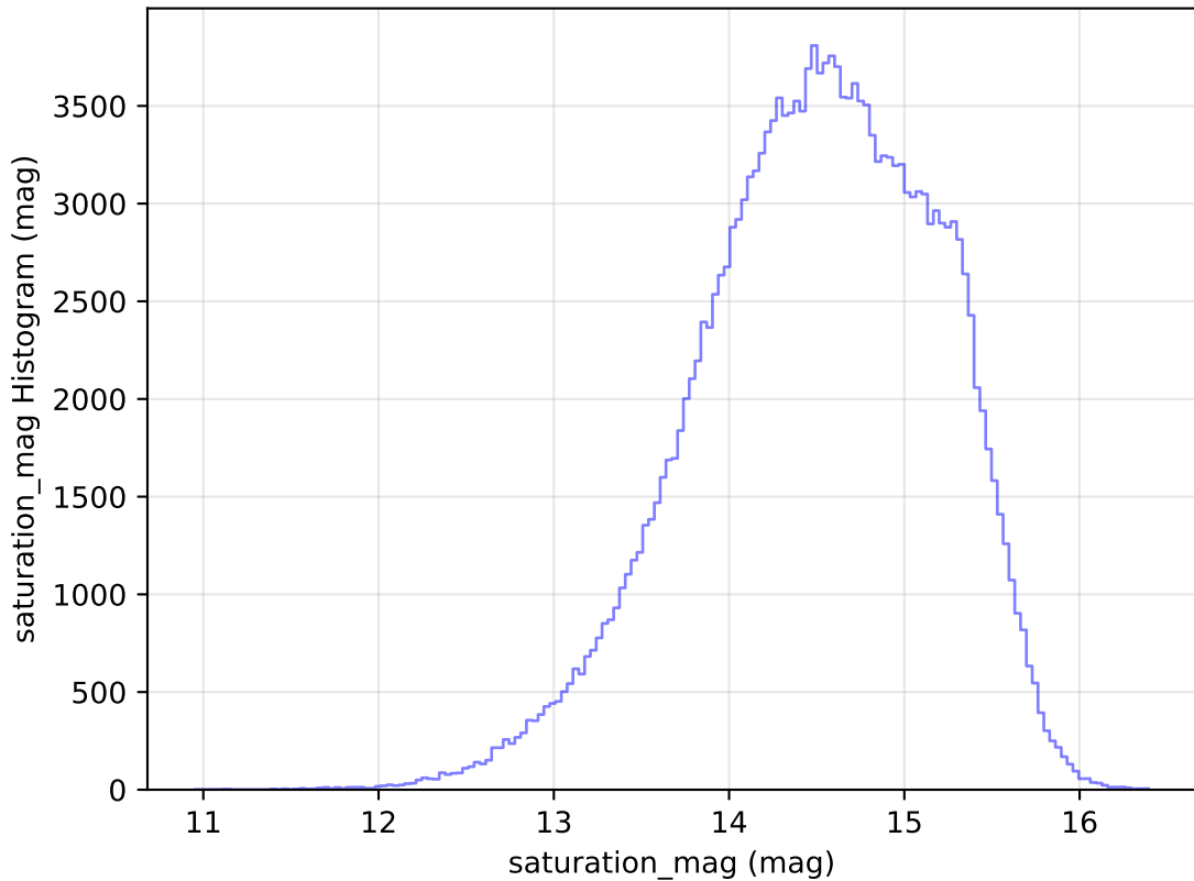
too_elab_r16_d2_giz_v3.4_10yrs WFD g band: saturation_mag Histogram
