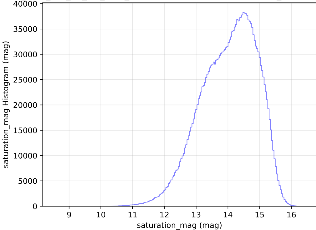
too_elab_r16_d2_giz_v3.4_10yrs WFD all bands: saturation_mag Histogram
