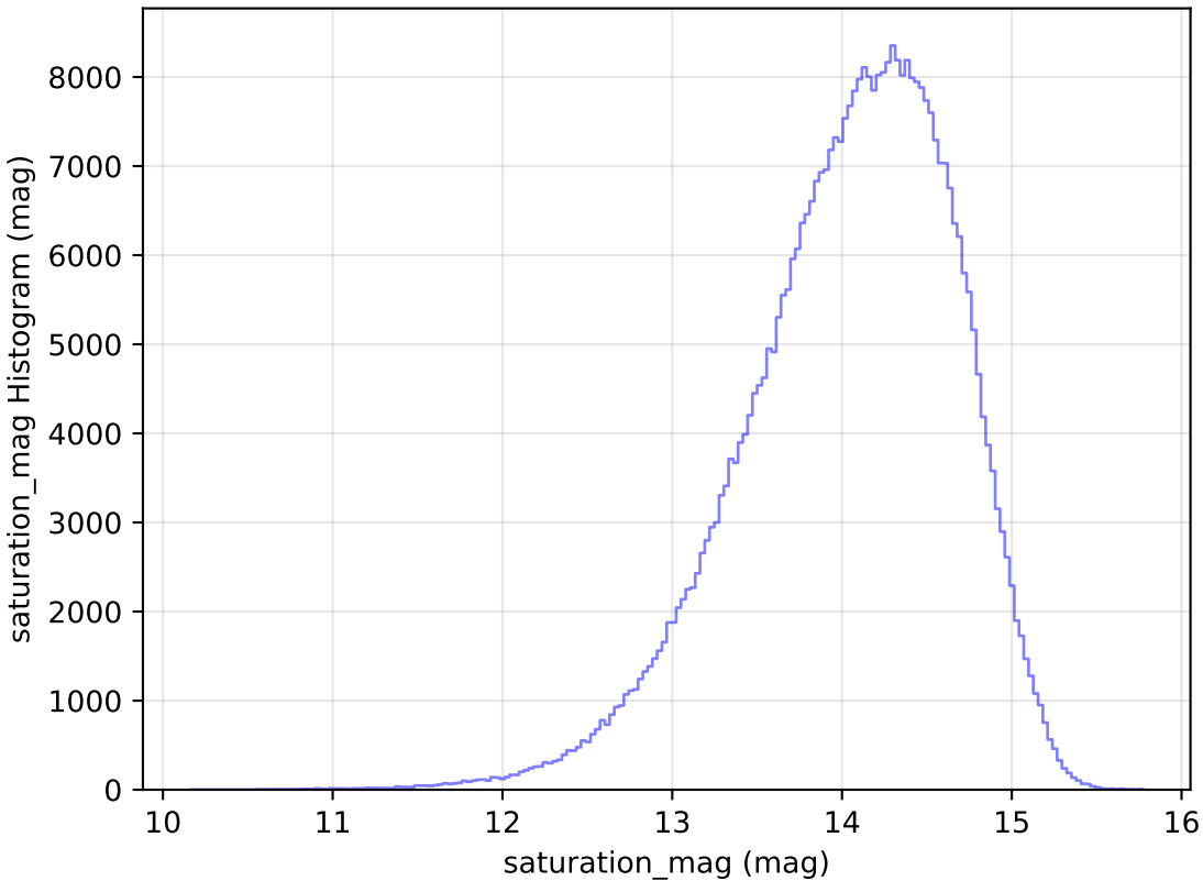
too_elab_r16_d2_giz_v3.4_10yrs All sky z band: saturation_mag Histogram
