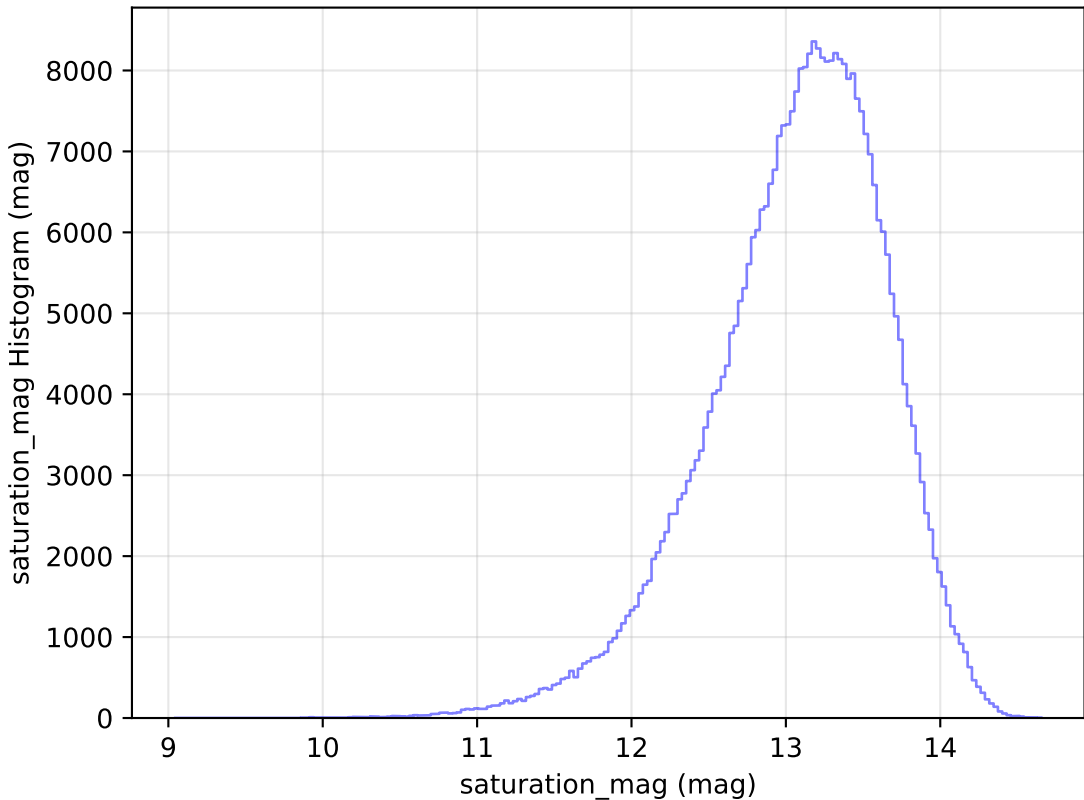
too_elab_r16_d2_giz_v3.4_10yrs All sky y band: saturation_mag Histogram
