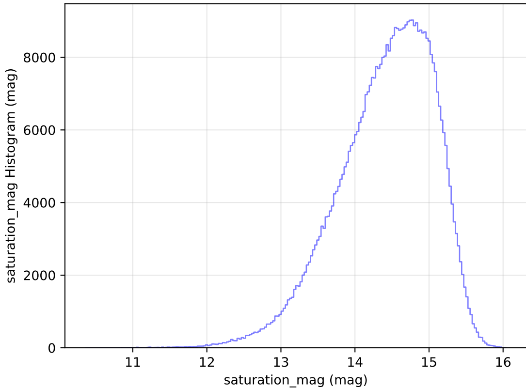
too_elab_r16_d2_giz_v3.4_10yrs All sky i band: saturation_mag Histogram
