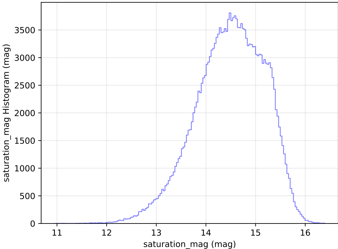
too_elab_r16_d2_giz_v3.4_10yrs All sky g band: saturation_mag Histogram
