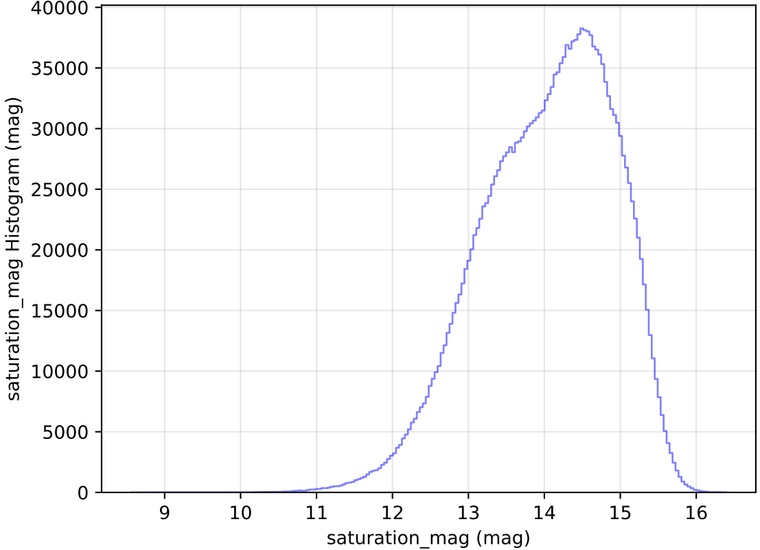
too_elab_r16_d2_giz_v3.4_10yrs All sky all bands: saturation_mag Histogram
