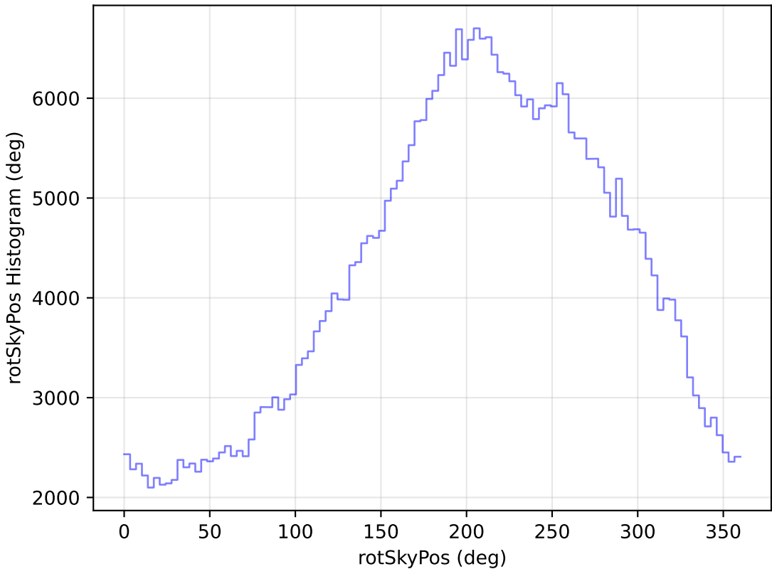
too_elab_r16_d2_giz_v3.4_10yrs WFD z band: rotSkyPos Histogram
