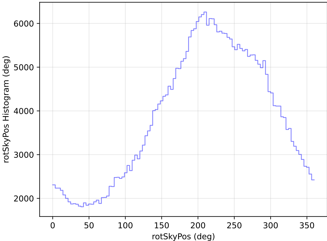
too_elab_r16_d2_giz_v3.4_10yrs WFD y band: rotSkyPos Histogram
