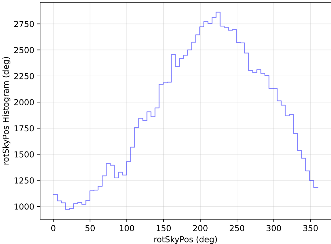
too_elab_r16_d2_giz_v3.4_10yrs WFD u band: rotSkyPos Histogram
