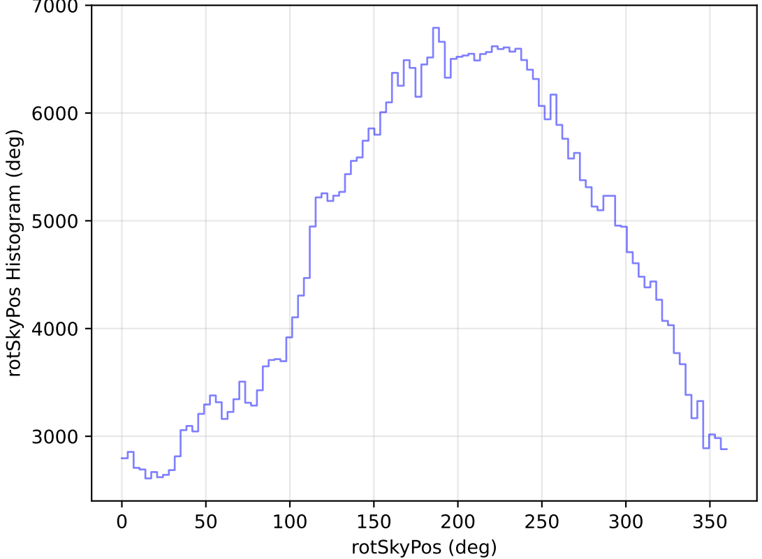
too_elab_r16_d2_giz_v3.4_10yrs WFD r band: rotSkyPos Histogram
