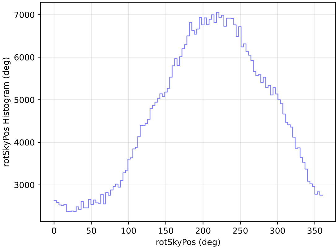
too_elab_r16_d2_giz_v3.4_10yrs WFD i band: rotSkyPos Histogram
