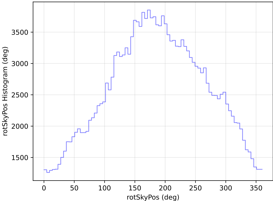
too_elab_r16_d2_giz_v3.4_10yrs WFD g band: rotSkyPos Histogram
