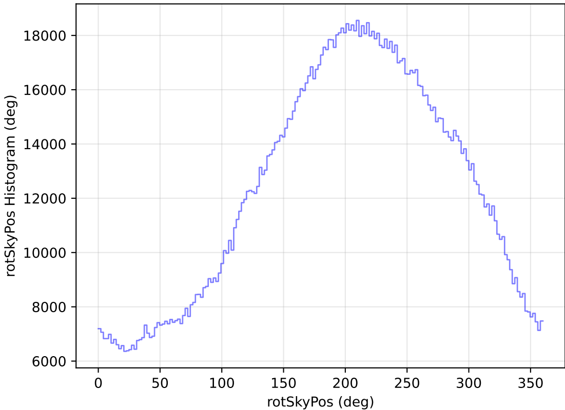
too_elab_r16_d2_giz_v3.4_10yrs WFD all bands: rotSkyPos Histogram
