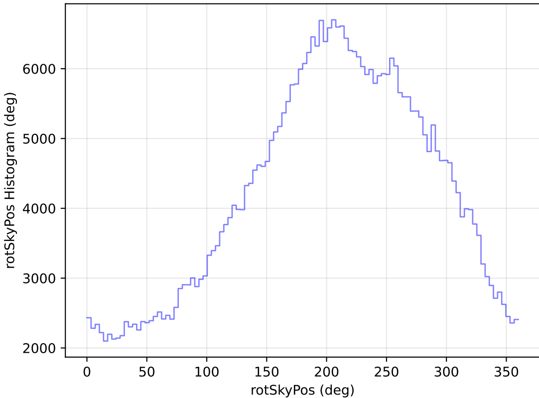
too_elab_r16_d2_giz_v3.4_10yrs All sky z band: rotSkyPos Histogram
