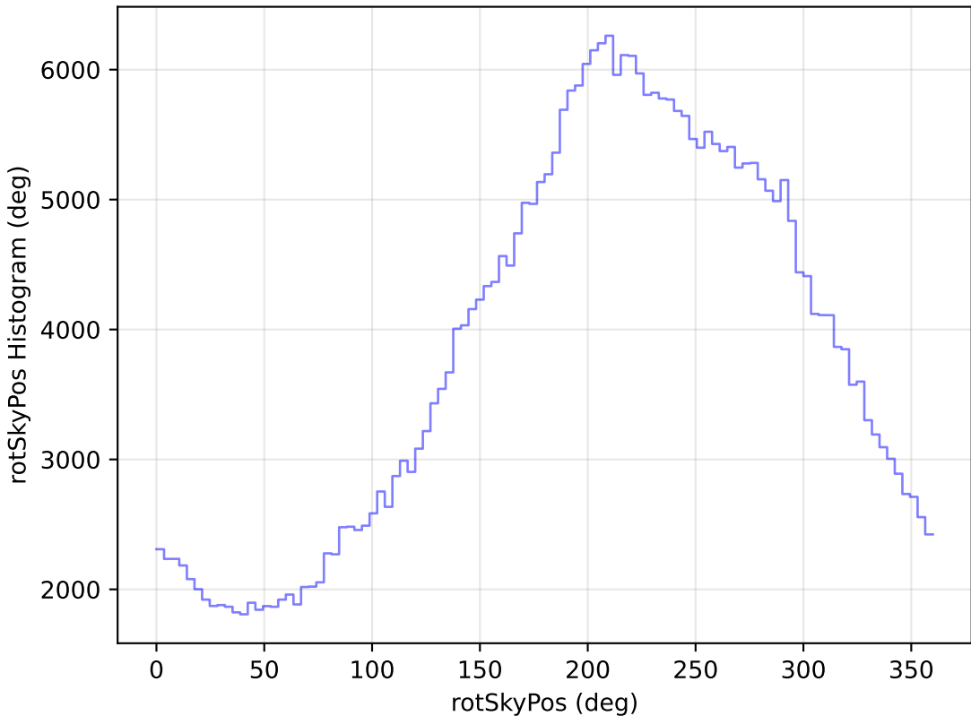
too_elab_r16_d2_giz_v3.4_10yrs All sky y band: rotSkyPos Histogram
