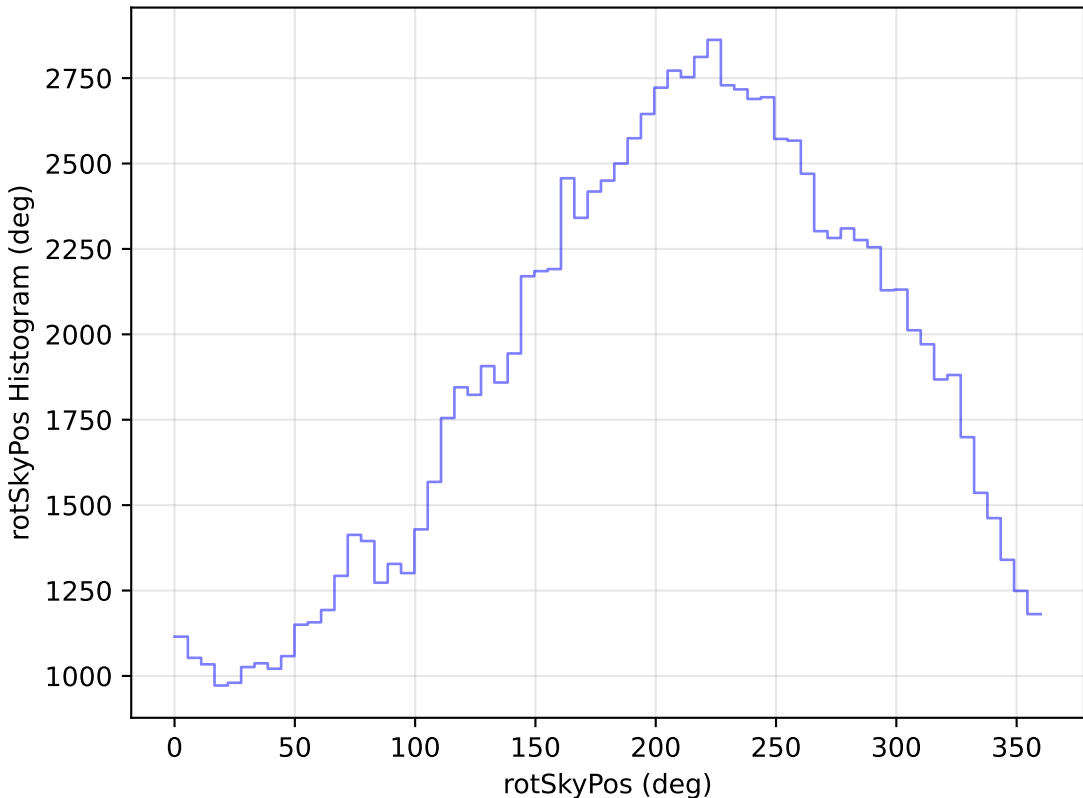
too_elab_r16_d2_giz_v3.4_10yrs All sky u band: rotSkyPos Histogram
