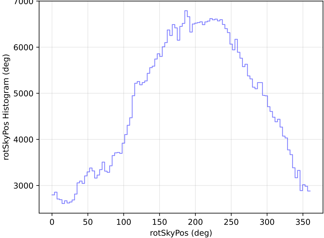
too_elab_r16_d2_giz_v3.4_10yrs All sky r band: rotSkyPos Histogram
