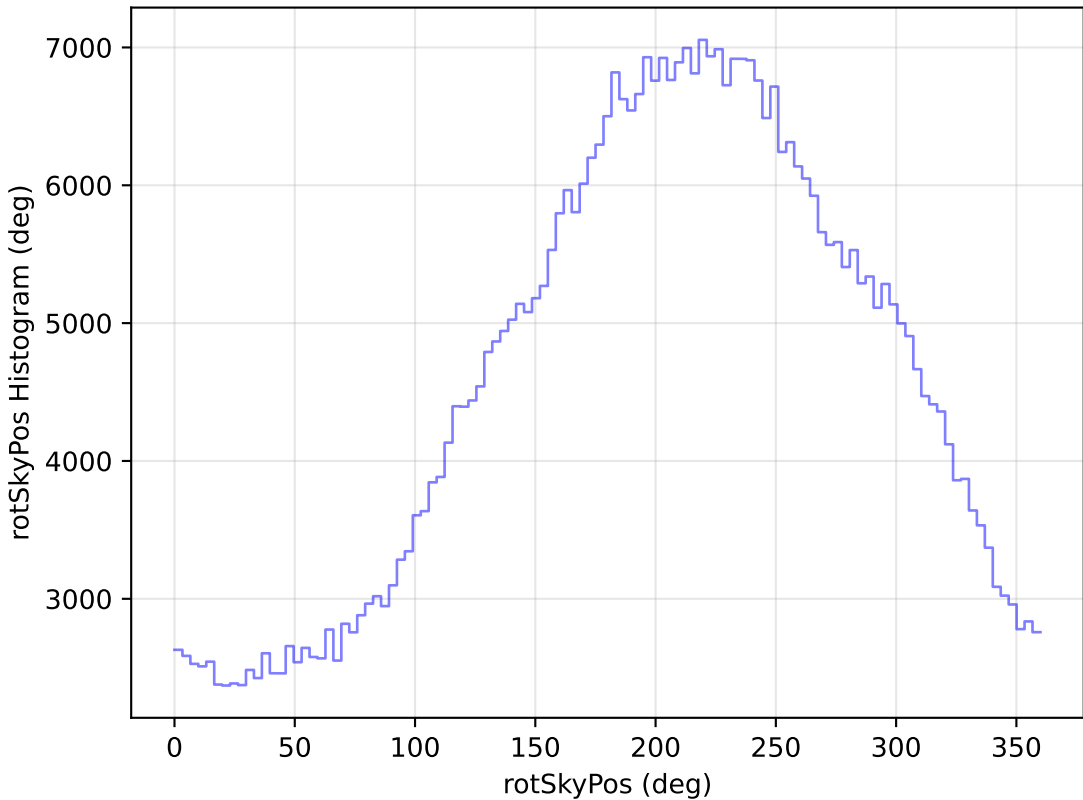
too_elab_r16_d2_giz_v3.4_10yrs All sky i band: rotSkyPos Histogram
