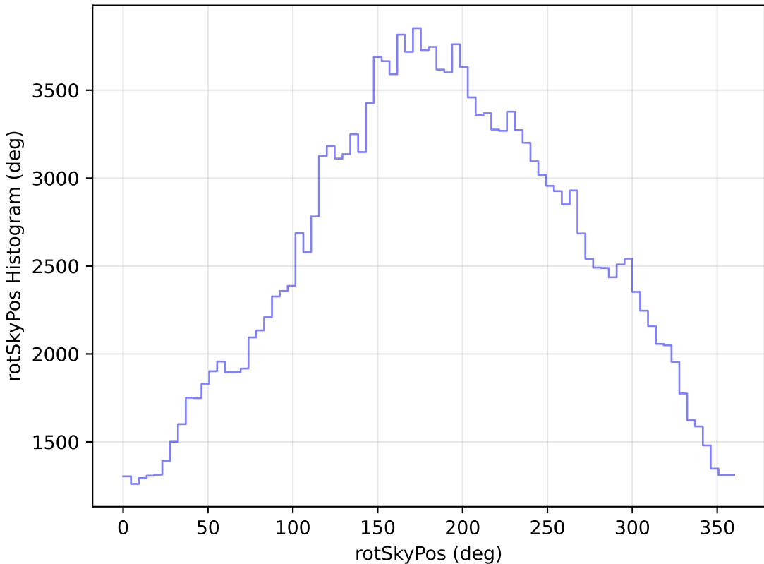
too_elab_r16_d2_giz_v3.4_10yrs All sky g band: rotSkyPos Histogram
