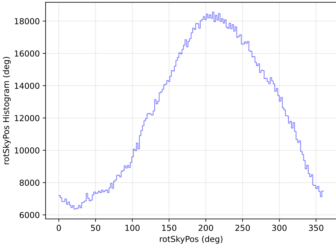
too_elab_r16_d2_giz_v3.4_10yrs All sky all bands: rotSkyPos Histogram
