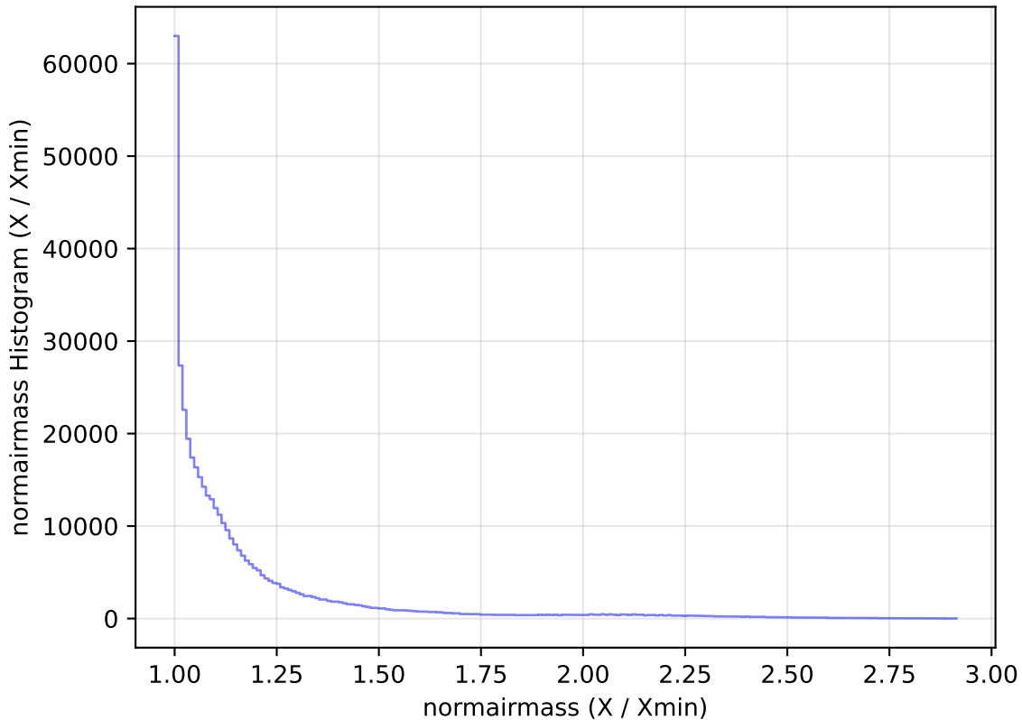
too_elab_r16_d2_giz_v3.4_10yrs WFD z band: normairmass Histogram
