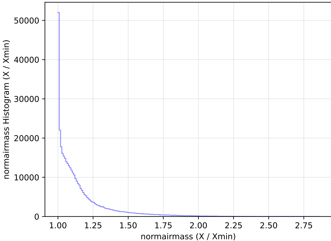
too_elab_r16_d2_giz_v3.4_10yrs WFD y band: normairmass Histogram
