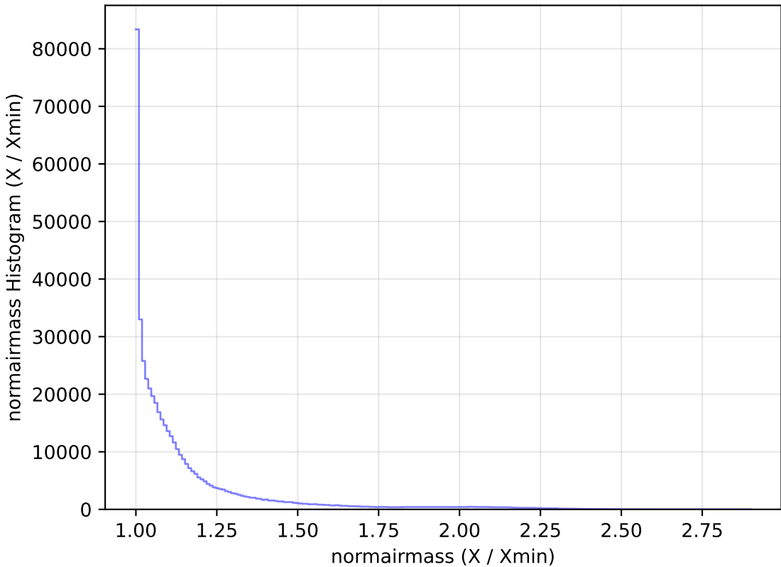
too_elab_r16_d2_giz_v3.4_10yrs WFD r band: normairmass Histogram
