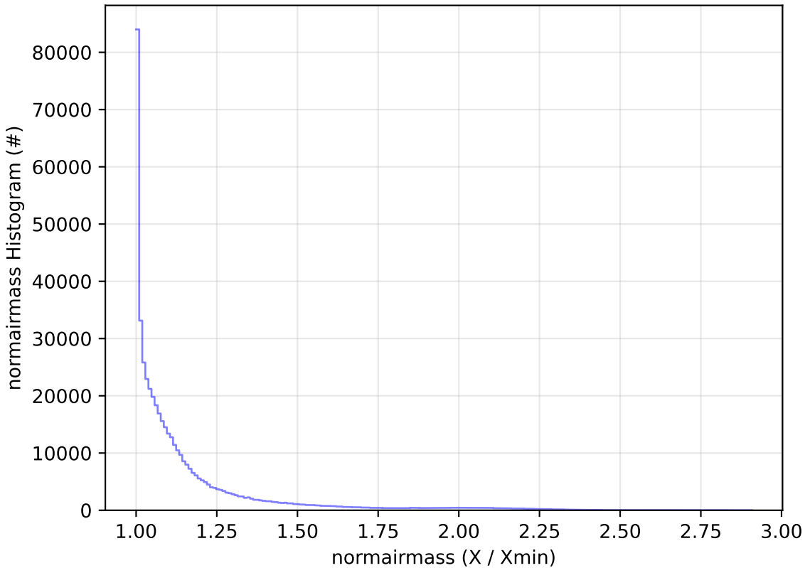
too_elab_r16_d2_giz_v3.4_10yrs WFD r band: normairmass Histogram
