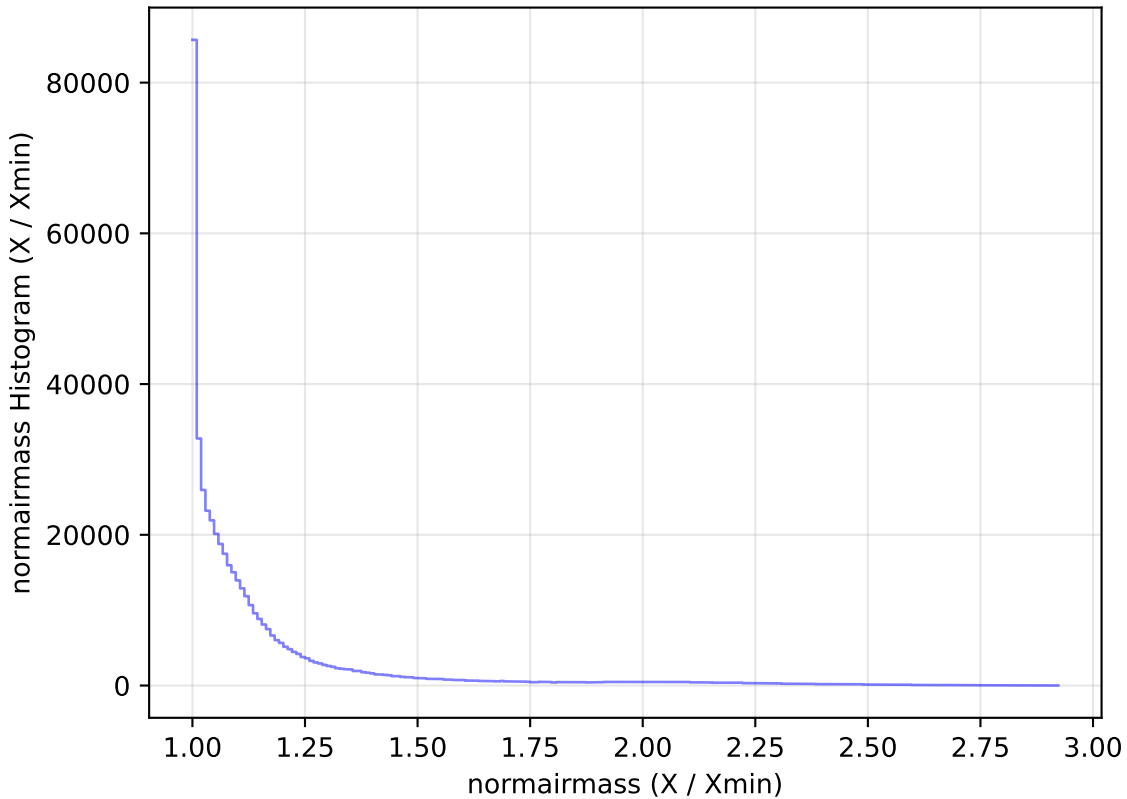
too_elab_r16_d2_giz_v3.4_10yrs WFD i band: normairmass Histogram
