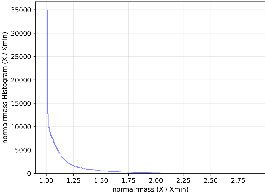
too_elab_r16_d2_giz_v3.4_10yrs WFD g band: normairmass Histogram
