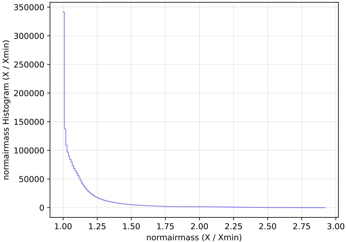
too_elab_r16_d2_giz_v3.4_10yrs WFD all bands: normairmass Histogram
