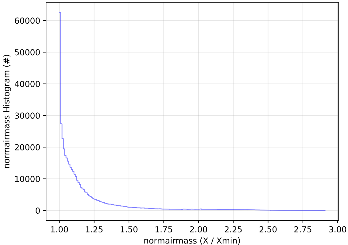
too_elab_r16_d2_giz_v3.4_10yrs All sky z band: normairmass Histogram
