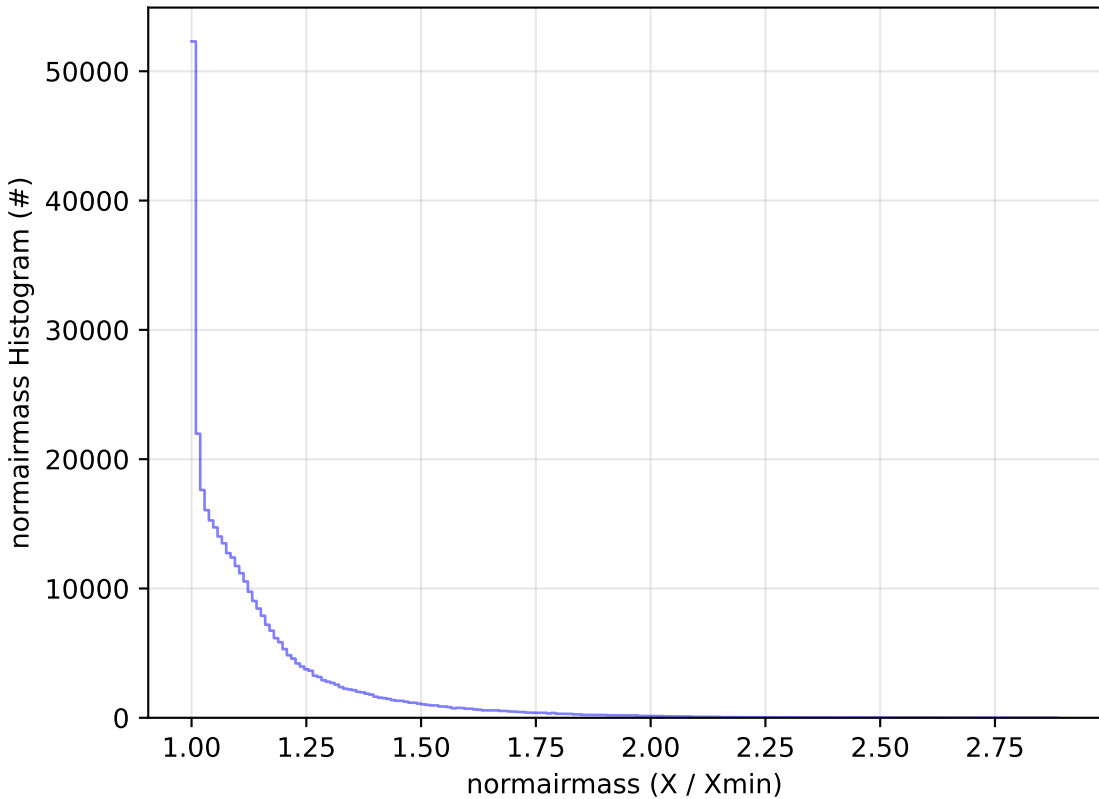
too_elab_r16_d2_giz_v3.4_10yrs All sky y band: normairmass Histogram
