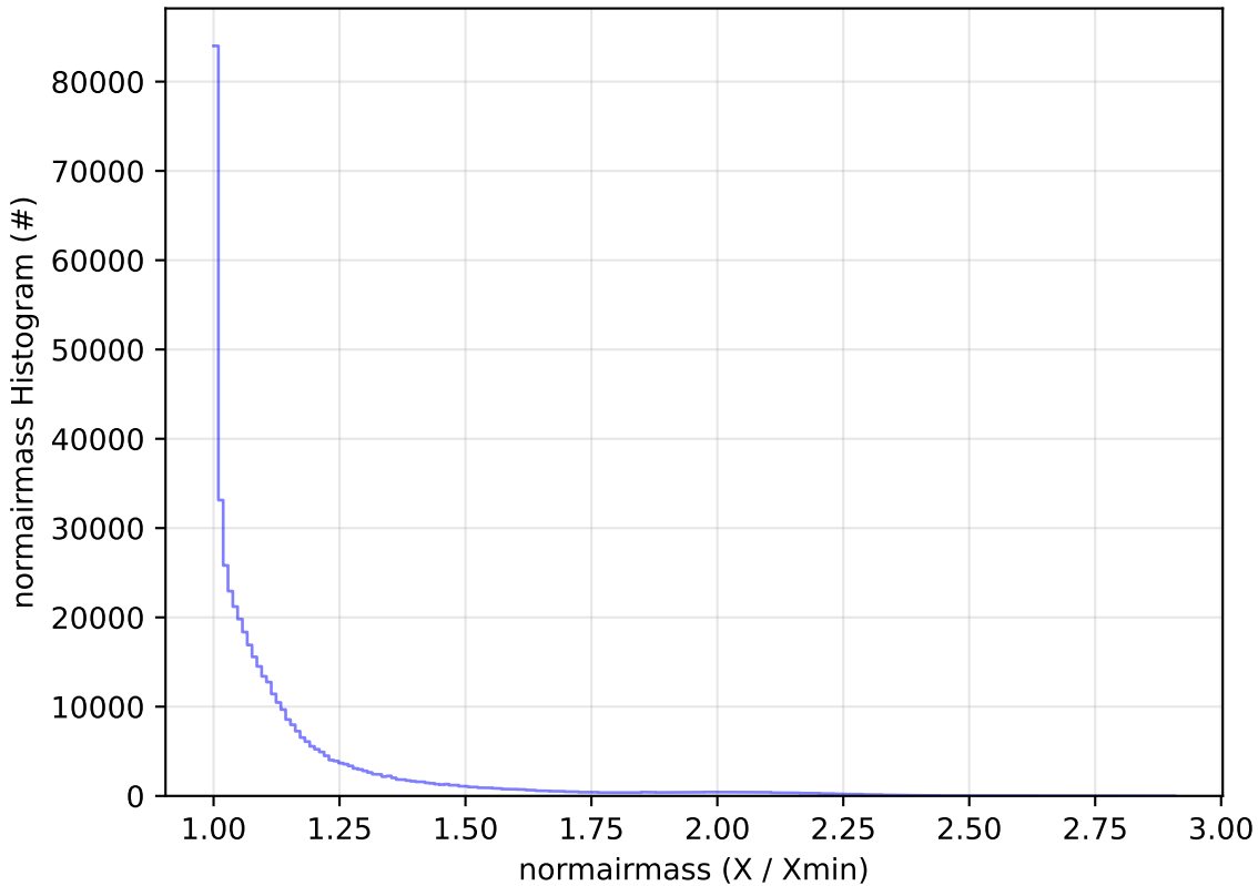
too_elab_r16_d2_giz_v3.4_10yrs All sky r band: normairmass Histogram
