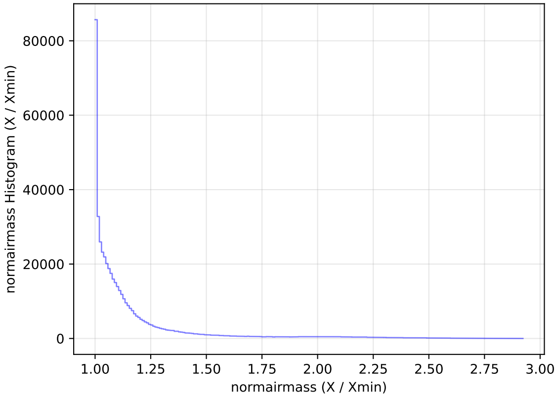
too_elab_r16_d2_giz_v3.4_10yrs All sky i band: normairmass Histogram
