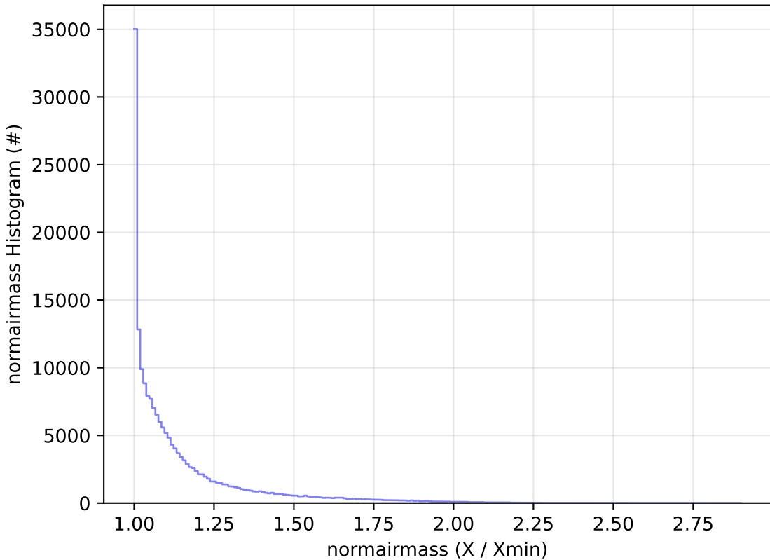
too_elab_r16_d2_giz_v3.4_10yrs All sky g band: normairmass Histogram
