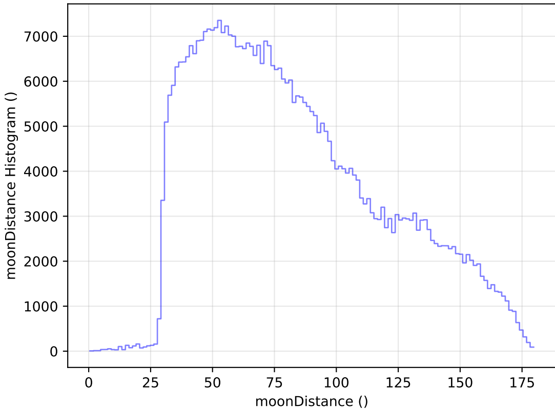
too_elab_r16_d2_giz_v3.4_10yrs WFD z band: moonDistance Histogram
