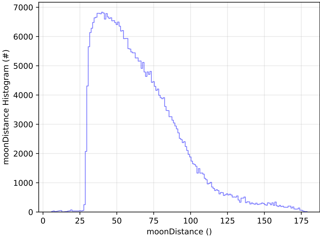
too_elab_r16_d2_giz_v3.4_10yrs WFD y band: moonDistance Histogram
