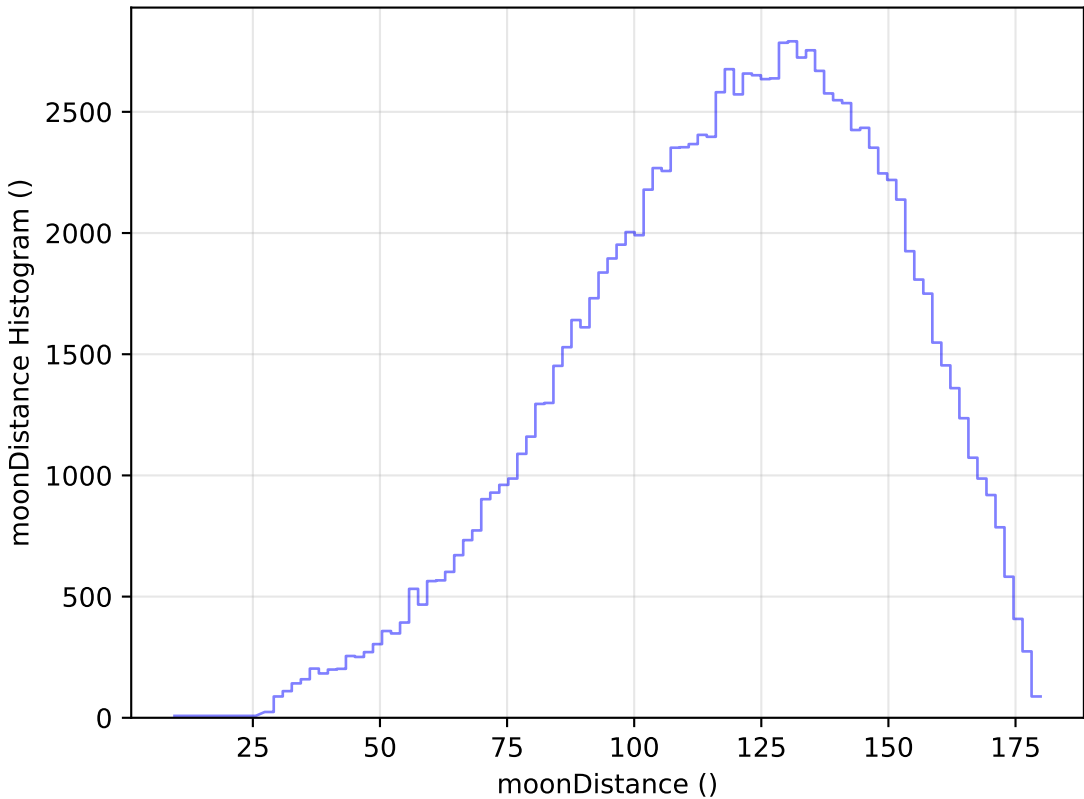
too_elab_r16_d2_giz_v3.4_10yrs WFD u band: moonDistance Histogram
