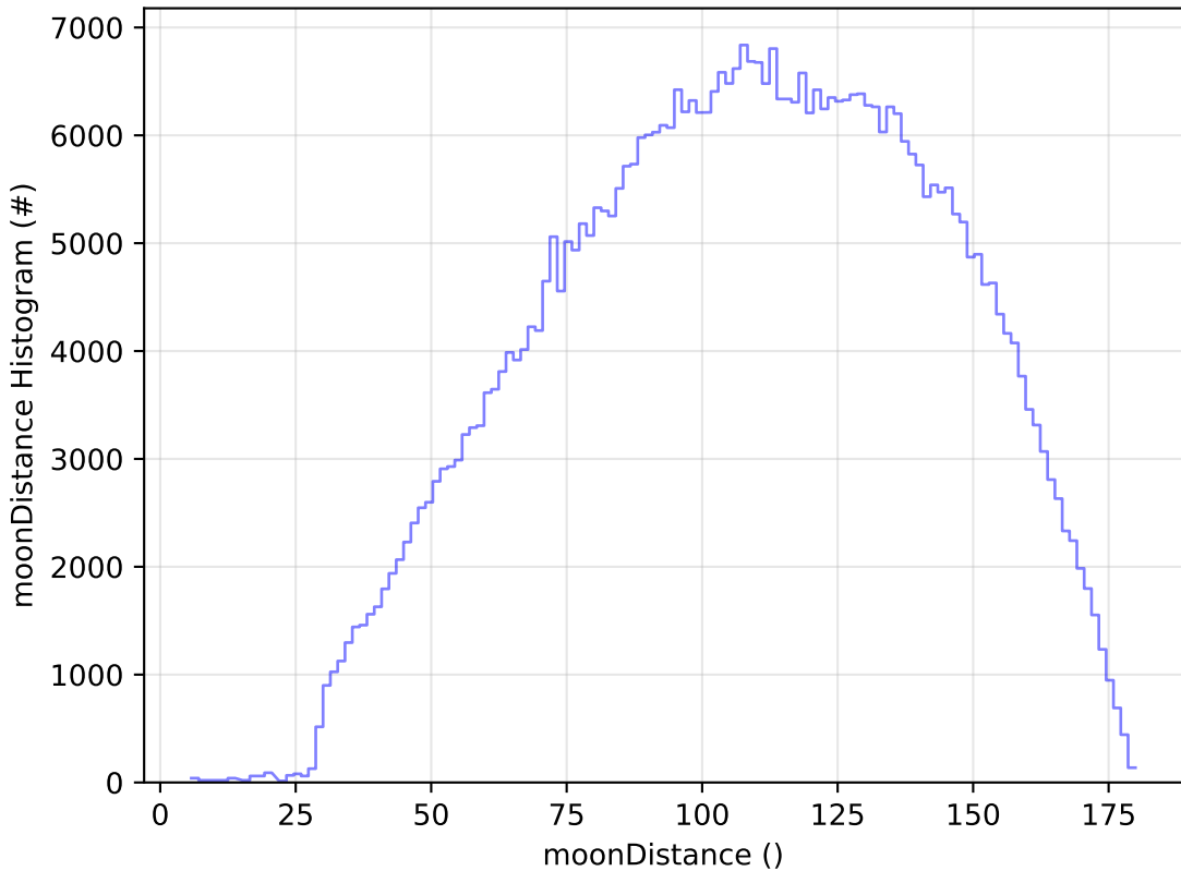
too_elab_r16_d2_giz_v3.4_10yrs WFD r band: moonDistance Histogram
