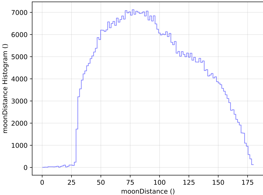
too_elab_r16_d2_giz_v3.4_10yrs WFD i band: moonDistance Histogram
