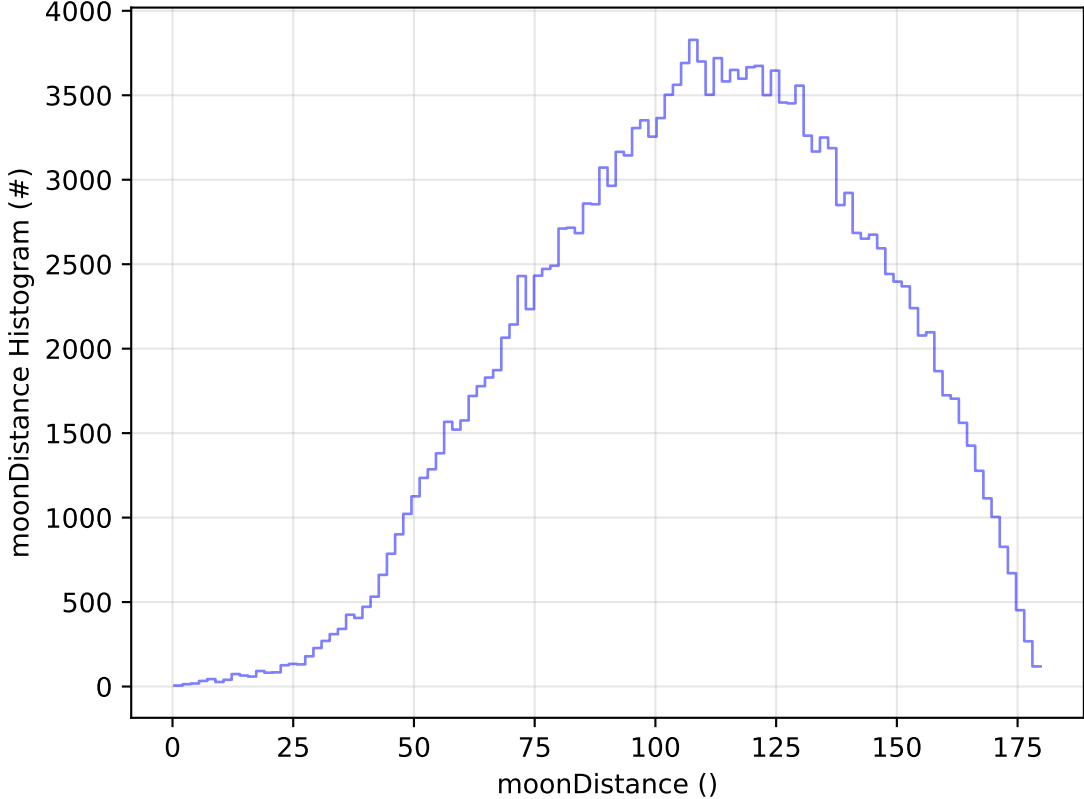
too_elab_r16_d2_giz_v3.4_10yrs WFD g band: moonDistance Histogram
