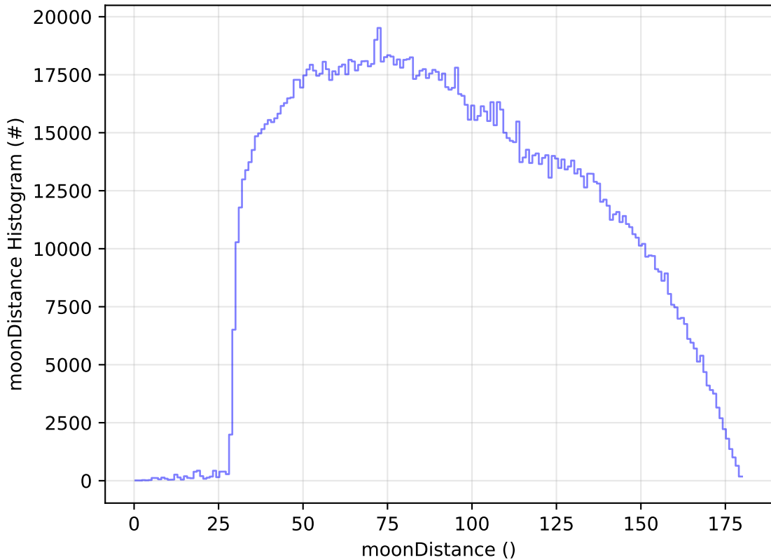
too_elab_r16_d2_giz_v3.4_10yrs WFD all bands: moonDistance Histogram
