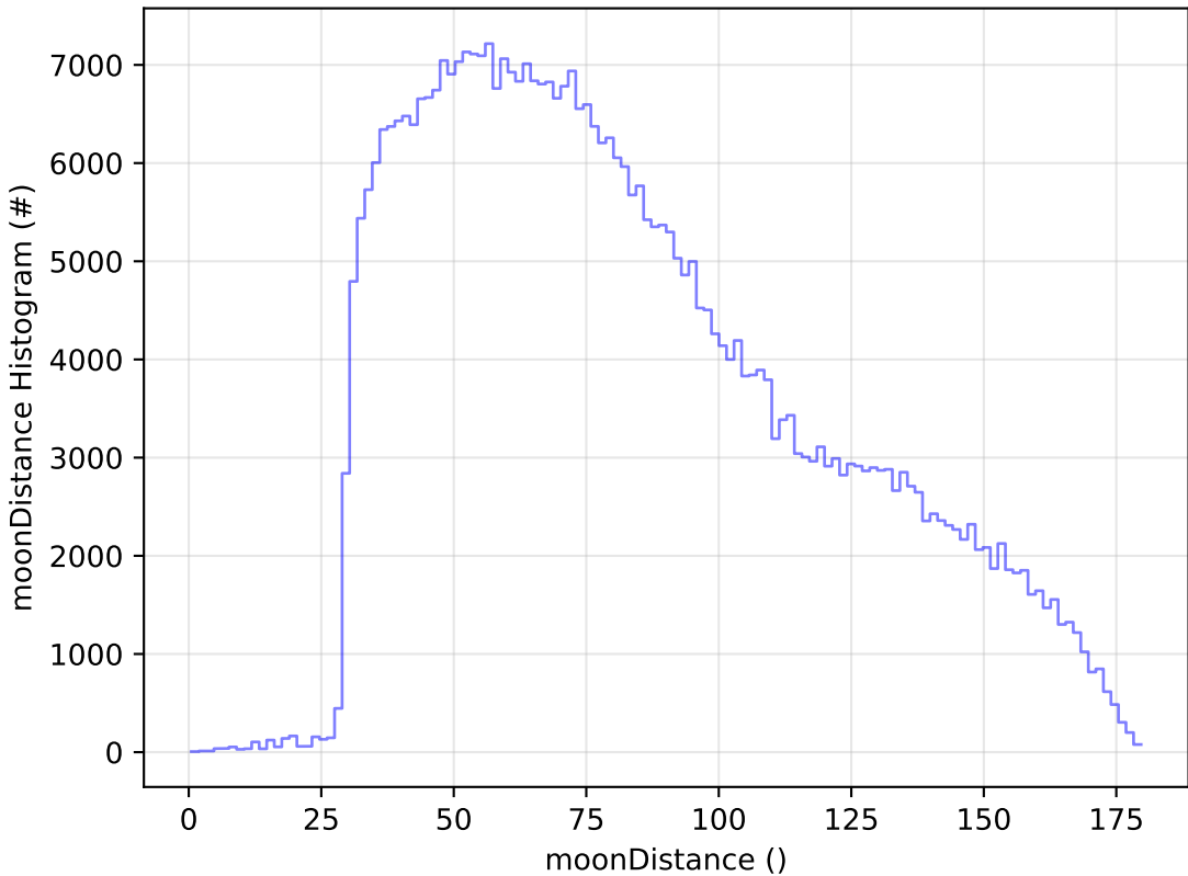
too_elab_r16_d2_giz_v3.4_10yrs All sky z band: moonDistance Histogram
