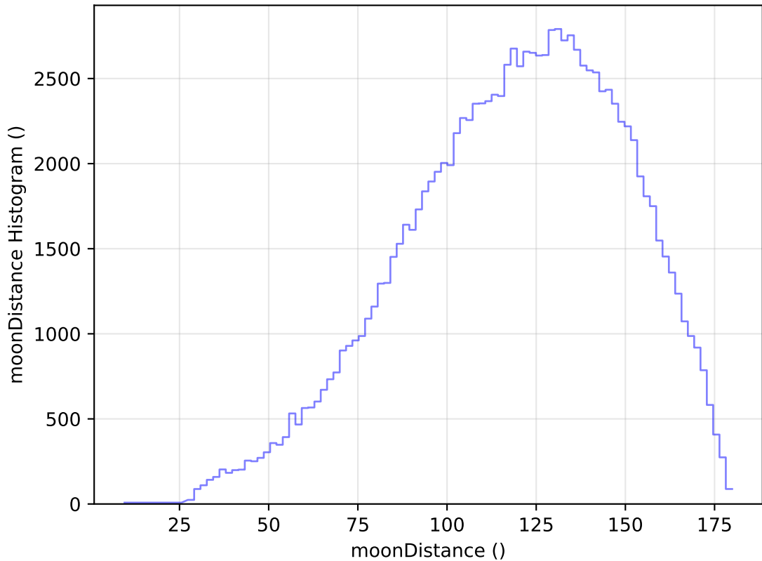
too_elab_r16_d2_giz_v3.4_10yrs All sky u band: moonDistance Histogram
