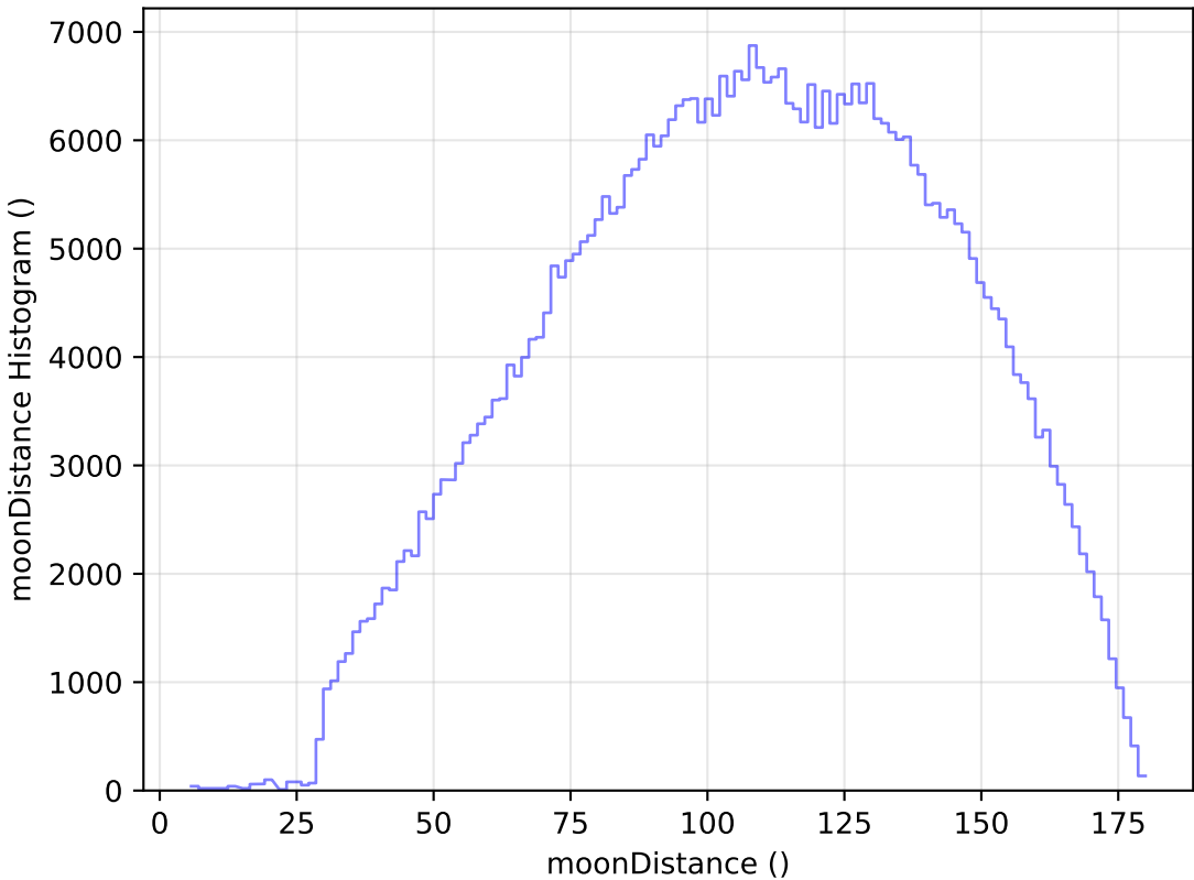
too_elab_r16_d2_giz_v3.4_10yrs All sky r band: moonDistance Histogram
