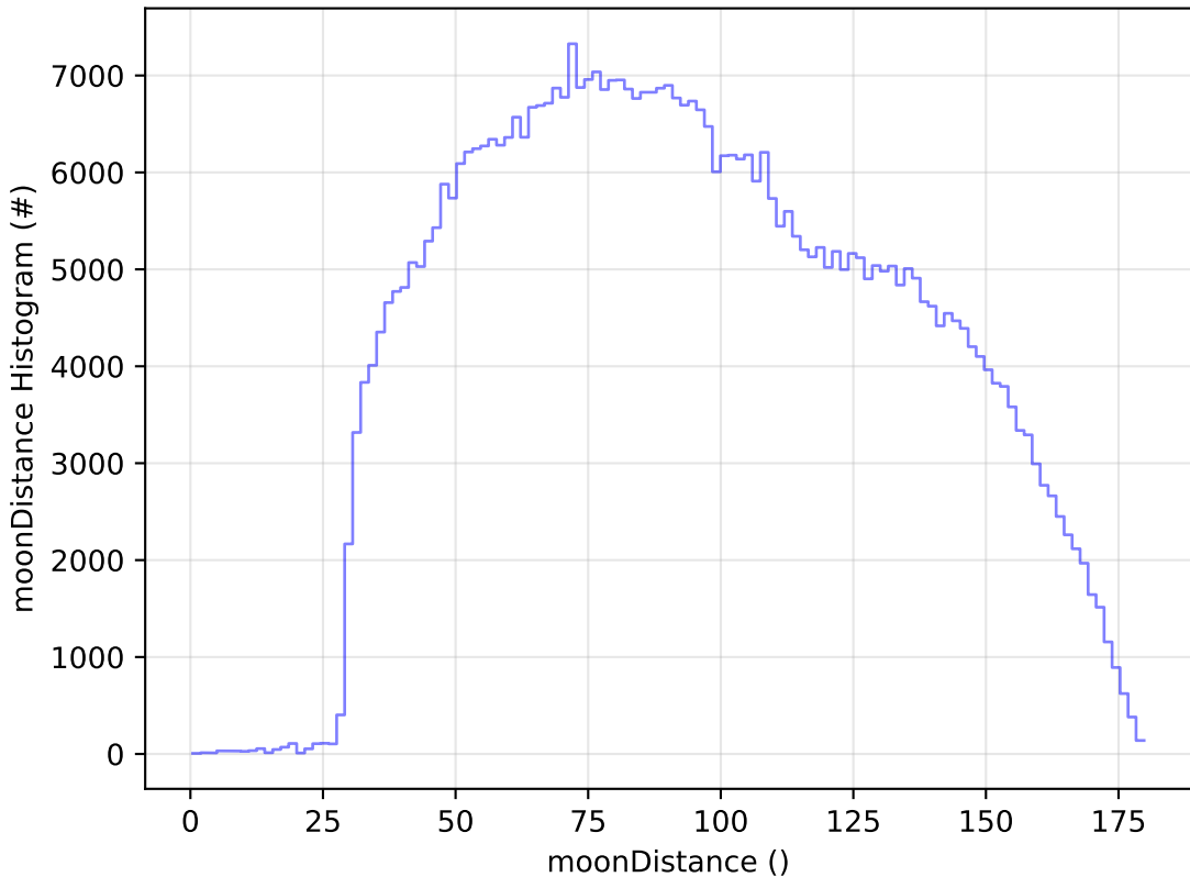
too_elab_r16_d2_giz_v3.4_10yrs All sky i band: moonDistance Histogram
