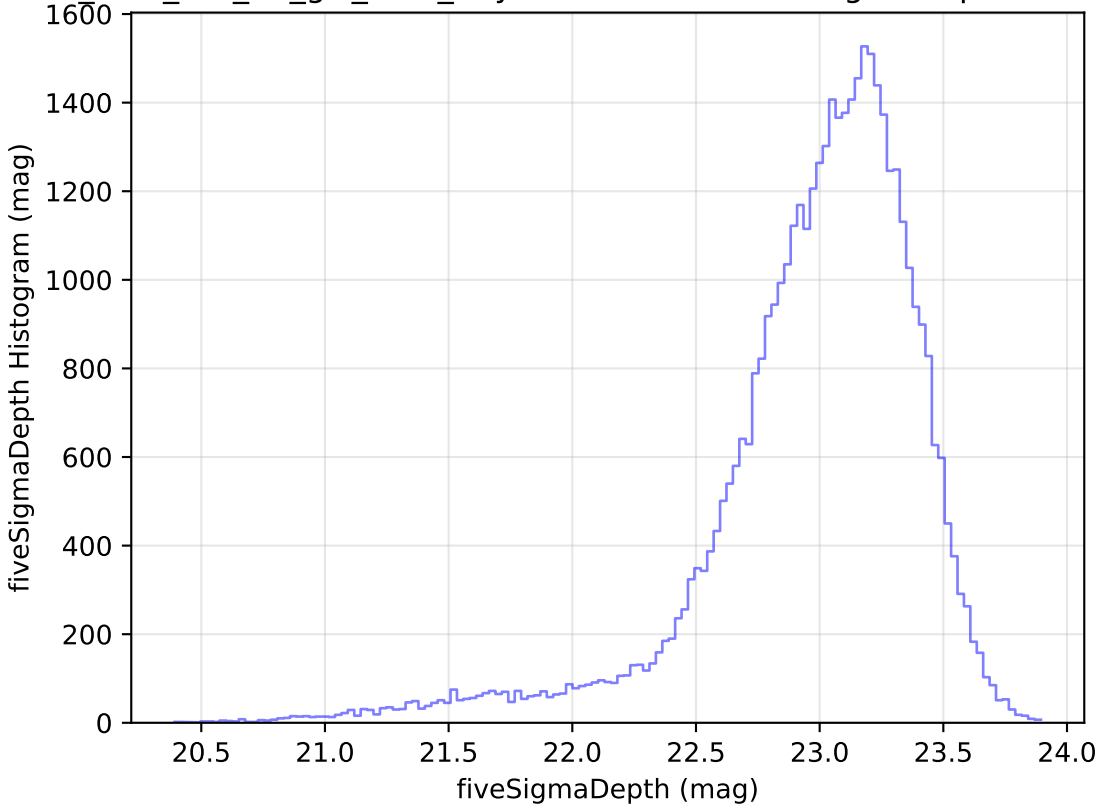
too_elab_r16_d2_giz_v3.4_10yrs Yr 1 z band: fiveSigmaDepth Histogram
