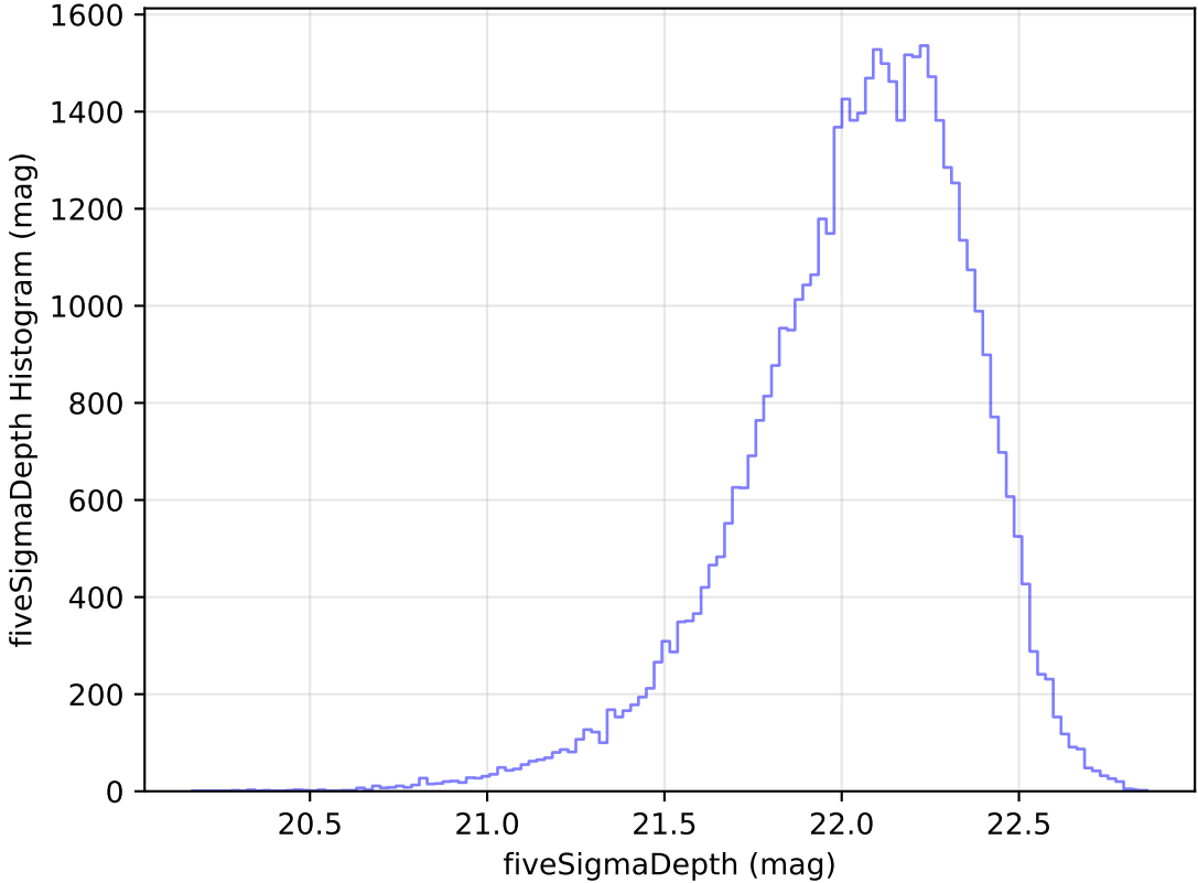
too_elab_r16_d2_giz_v3.4_10yrs Yr 1 y band: fiveSigmaDepth Histogram
