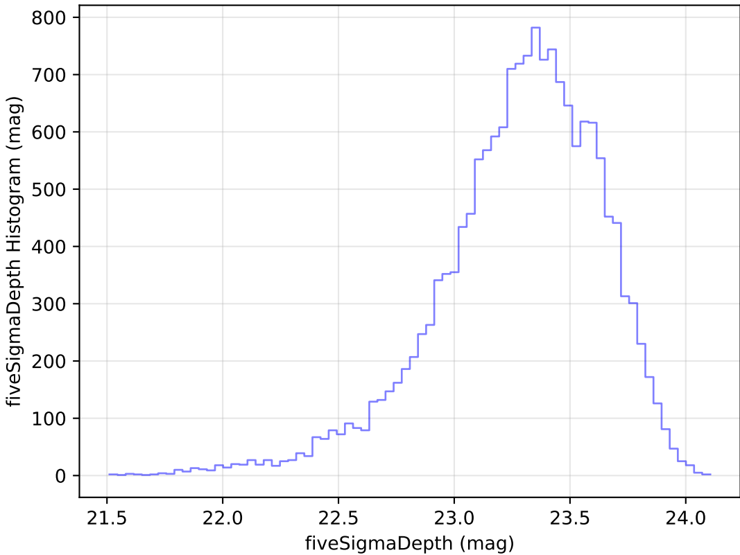
too_elab_r16_d2_giz_v3.4_10yrs Yr 1 u band: fiveSigmaDepth Histogram
