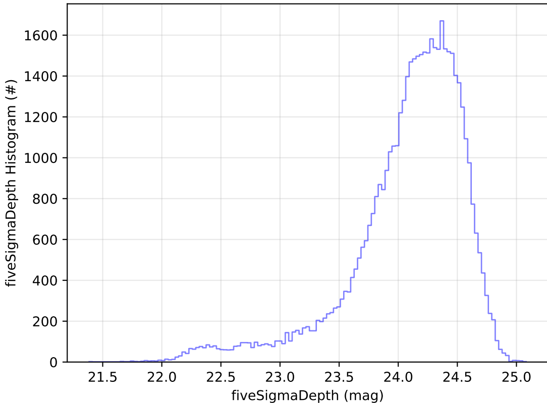
too_elab_r16_d2_giz_v3.4_10yrs Yr 1 r band: fiveSigmaDepth Histogram
